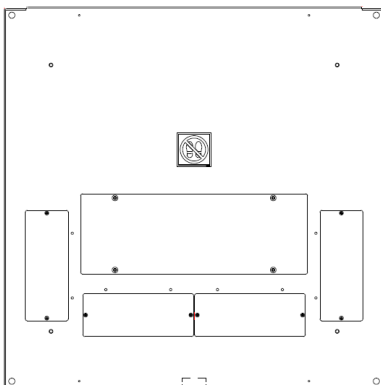
Top Panel 1off 448 x 130 4off 203 x 76
